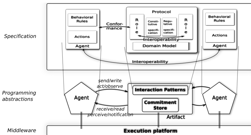
Fig. 1. The MERCURIO architecture.
